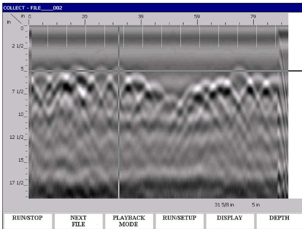
Figure 26: Data Collection screen in StructureScan Standard/Optical.
