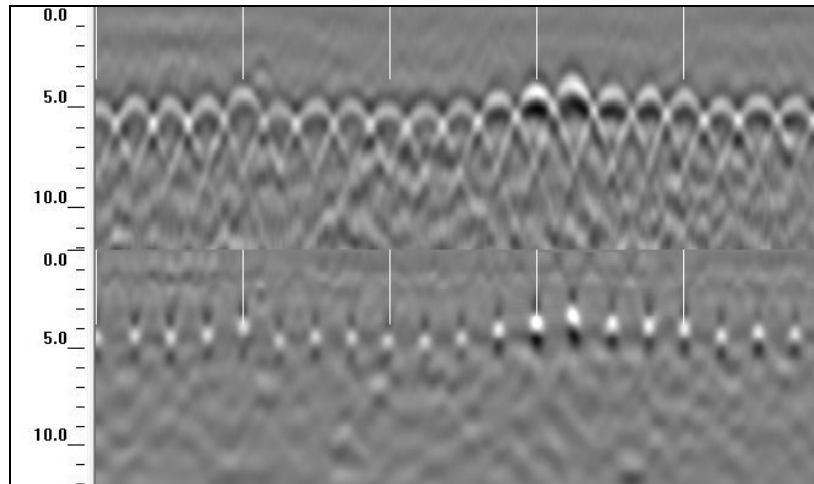
Figure 22: Raw and migrated data.
