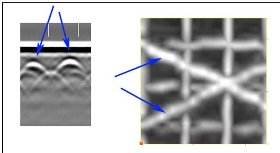
Figure 11: Two cables located above the rebar mat – vertical profile and plan view.
