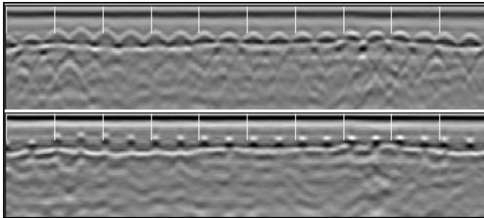
Figure 23: Unmigrated (top) and migrated (bottom) profiles of a concrete floor.
