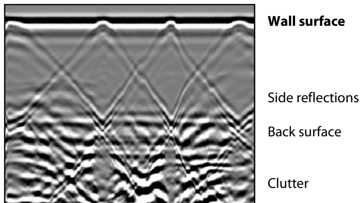
Figure 15: Interference patterns in radar data collected on a hollow wall with steel studs.
