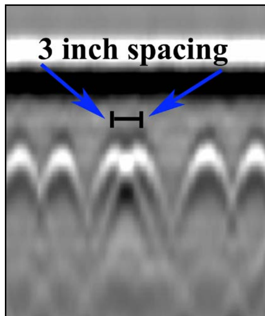
Figure 6: Two cables 3" apart (top left)
