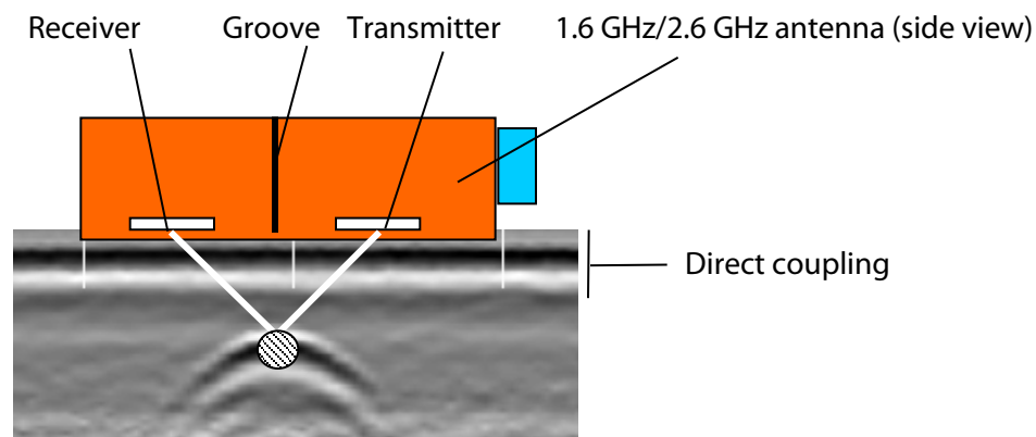
Figure 4: Locating a target.
