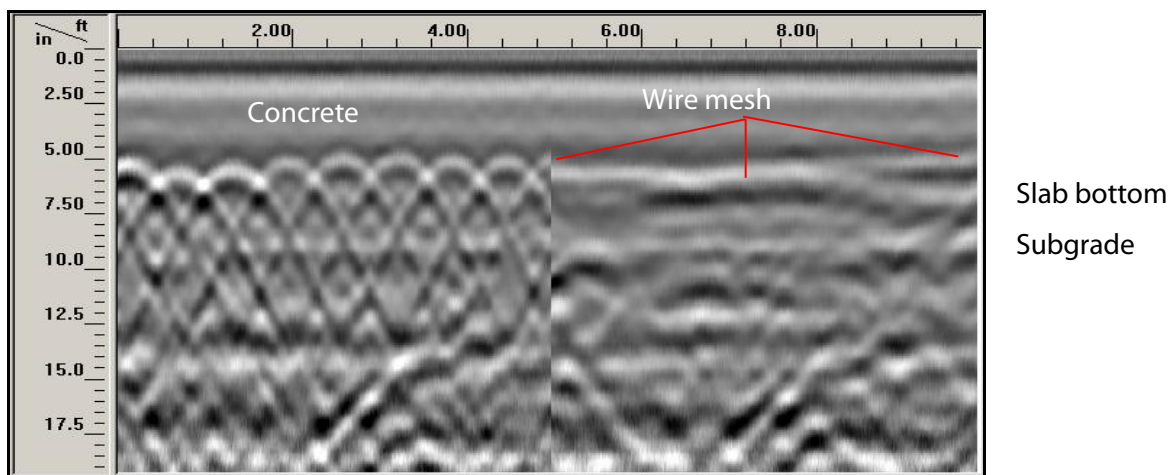
Figure 17: Slab on grade with a wire mesh. Left half of the profile - "standard" antenna position. Right half - same survey line with antenna turned sideways.
