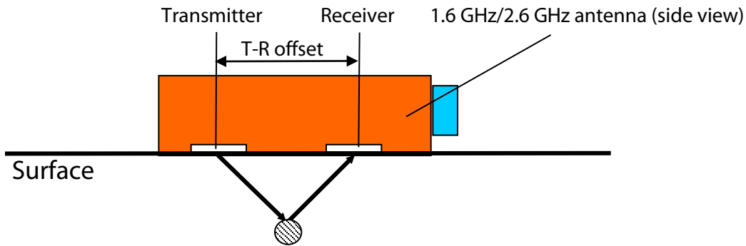
Figure 1: Antenna configuration.
