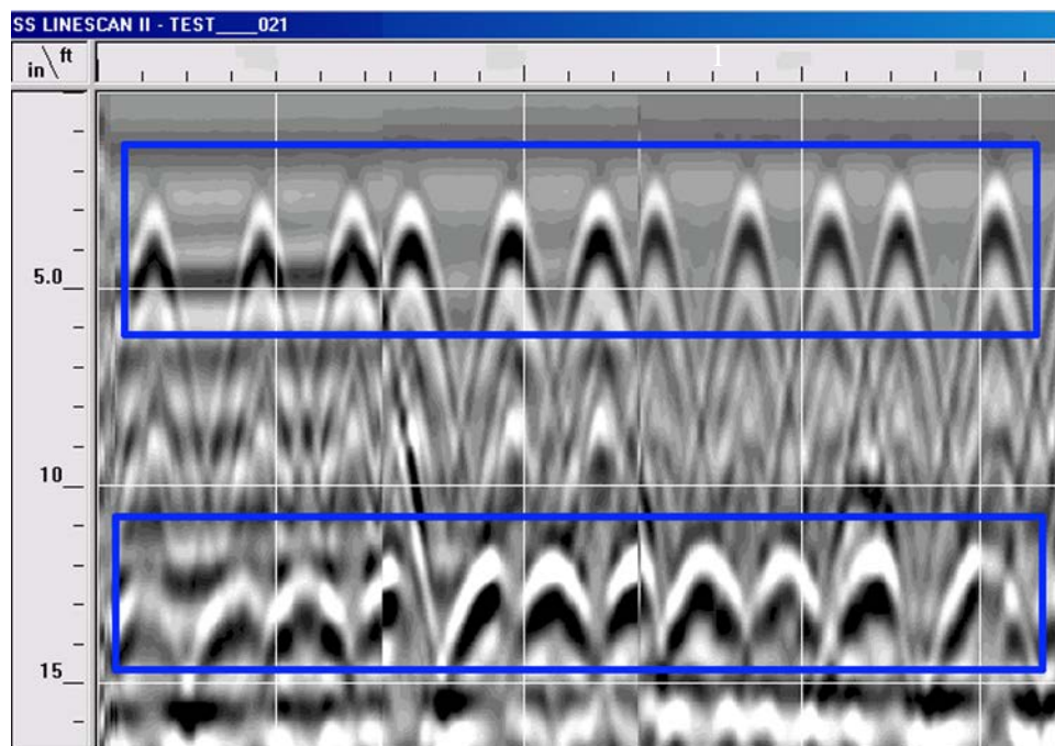
Figure 7: Two closely spaced layers of rebar.
