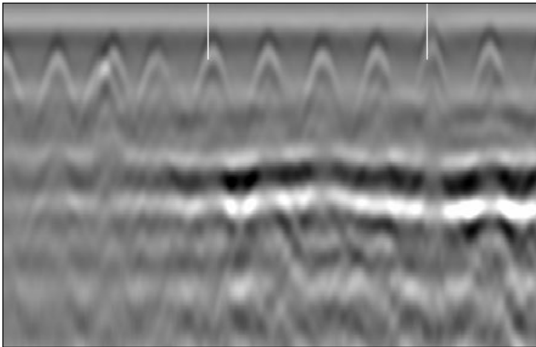
Figure 13: Example of void in concrete.
