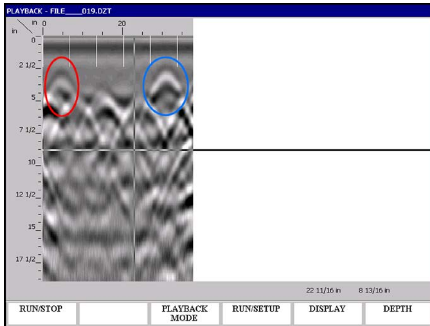
Figure 12: A metal (blue) and PVC (red) pipes of similar size at approximately the same depth.
