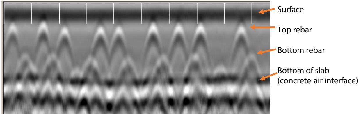
Figure 10: Two rebar mats (Elevated slab - balcony).
