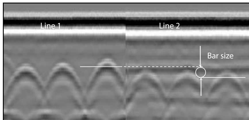
Figure 18: Rebar size measurement using two intersecting survey lines.
