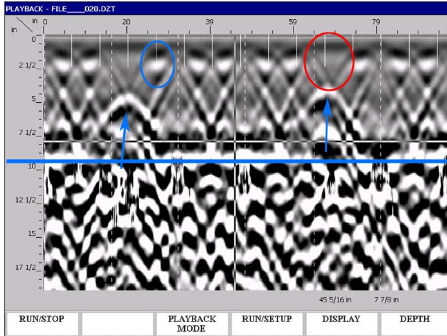
Figure 14: Masonry Blocks. Filled cell in red, hollow in blue.
