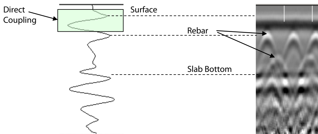
Figure 8: Oscilloscope (left) and Linescan displays of a reinforced balcony.
