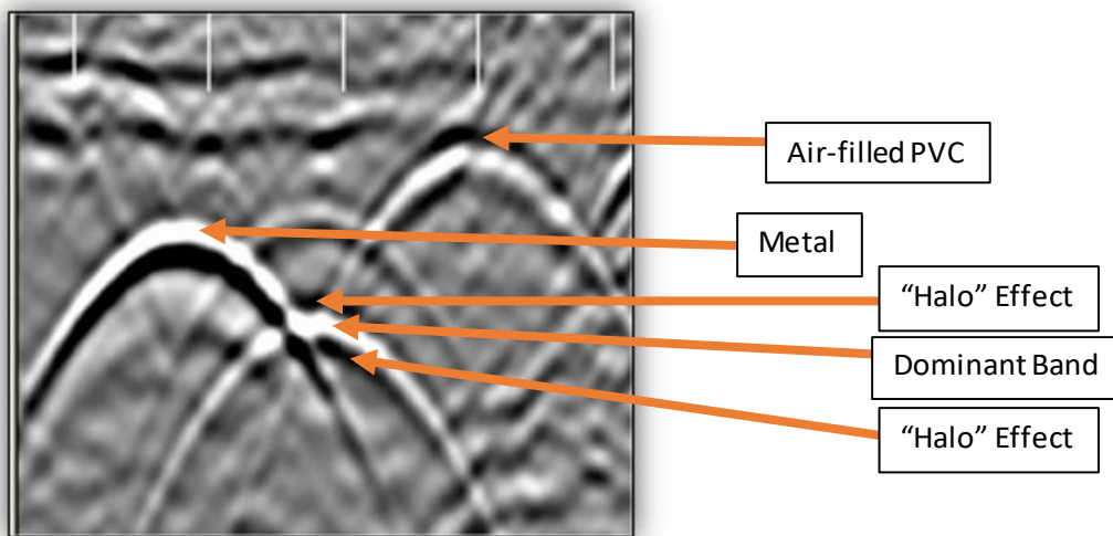
Figure 4: Metal and PVC targets. Reflection polarity.
