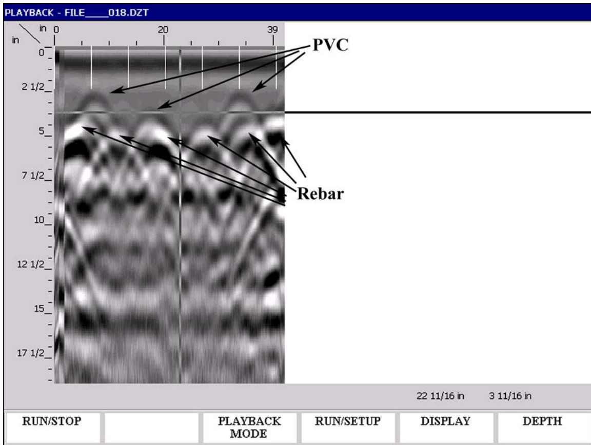
Figure 5: Hyperbolic reflections.
