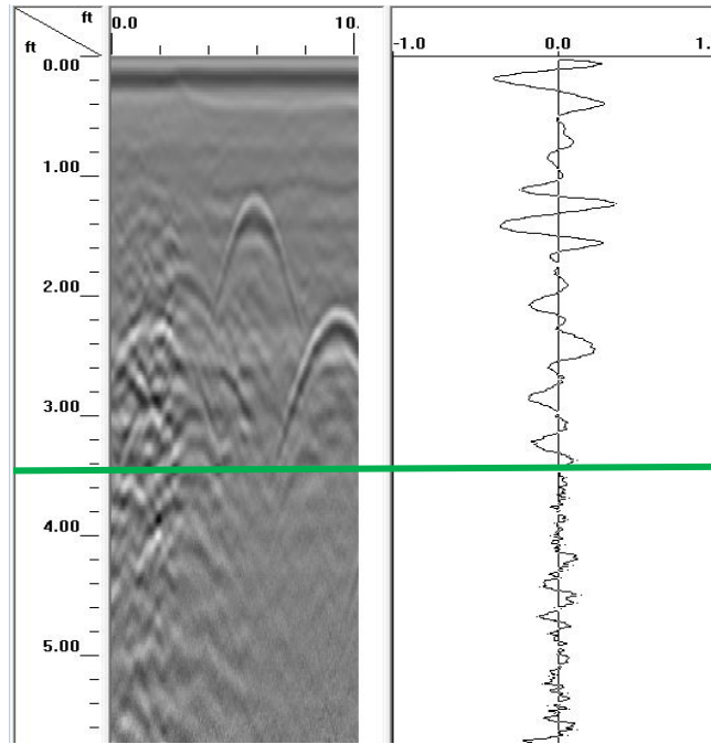
Figure 19: Linescan and O-scope of the same profile showing the penetration depth (green).
