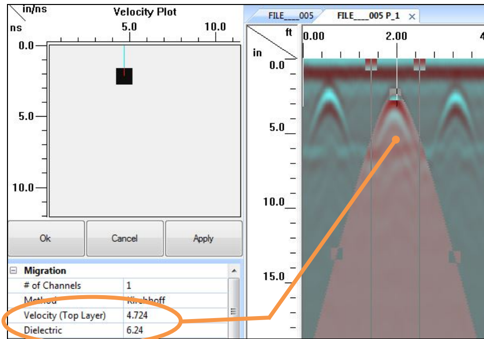
Figure 21: Velocity measurement in Migration.
