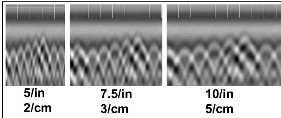
Figure 20: Scan spacing effects.
