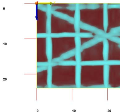
Figure 29: Depth Slice display of a 2 x 2 ft area showing the rebar mat with diagonal conduits.
