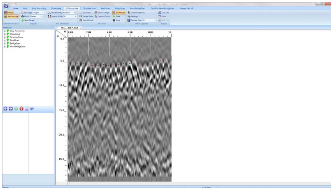
Figure 28: Data display in using 2D Interactive features.
