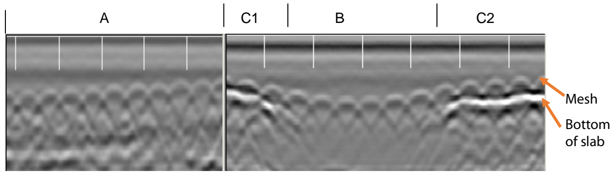
Figure 9: Concrete floor with a 6" wire mesh. The concrete bottom is just under the mesh.
